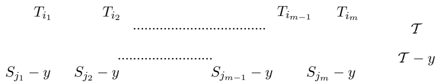
FIGURE 1. A geometric balanced pair in \mathcal{T} and \mathcal{T} - y .
